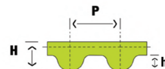
S-type tooth single sided profile
