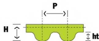
H-type tooth single sided profile
