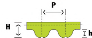
R-type tooth single sided profile
